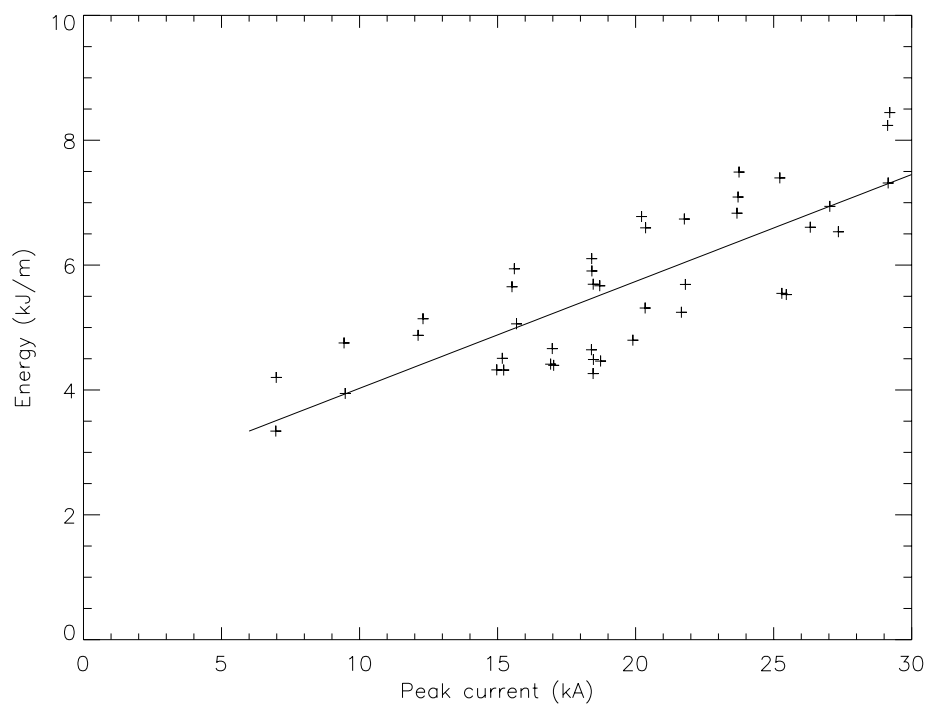
Figure 5: Energy dissipated as a function of peak current for the same data set in Figs. 4 and 3.
