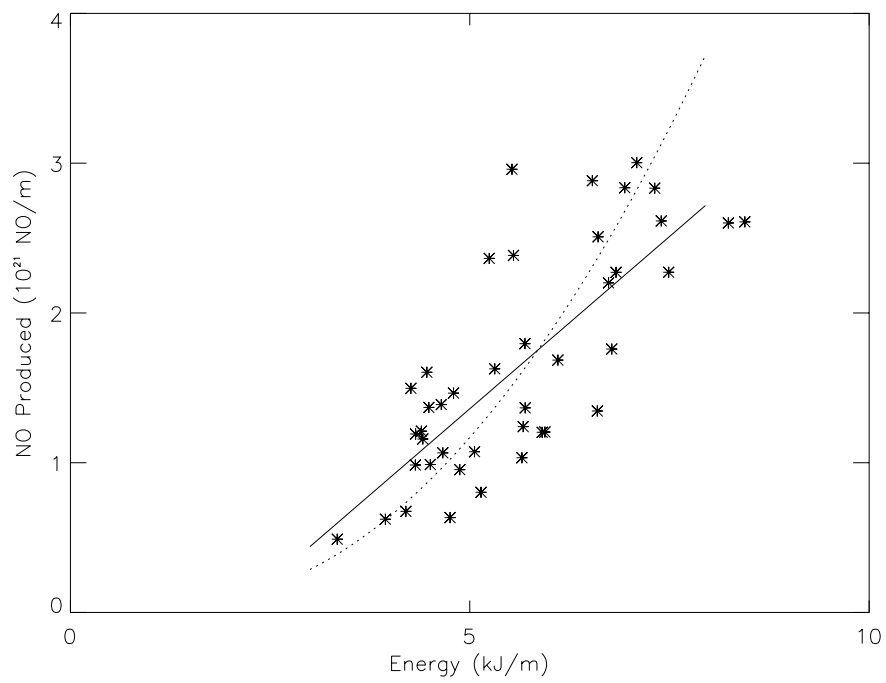
Figure 3: NO production as a function of dissipated energy in a spark, normalized to one meter spark length. The solid line is a linear least squares fit to the data. The dotted line is a quadratic representation derived from fits in Figs. 4 and 5.
