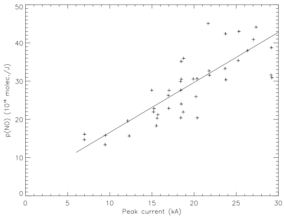
Figure 12: NO production divided by the energy dissipated, p(NO) , as a function of peak current.
