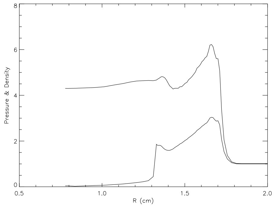
Figure 10: Simulation code results for the normalized pressure (top) and mass density (bottom) for the same case as Fig. 8.
